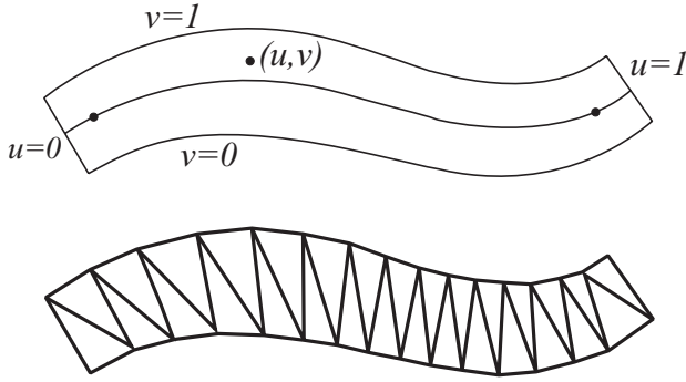
Figure 2: Top : Stroke model and texture coordinates. Bottom : Stroke tessellation as a triangle strip.
